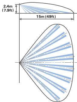
Coverage Pattern
