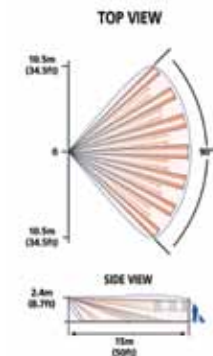
Coverage Pattern
